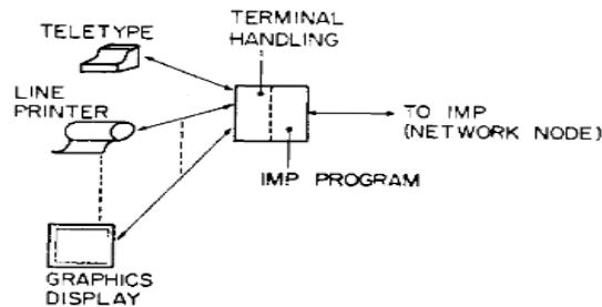
Fig. 2. Terminal IMP.
